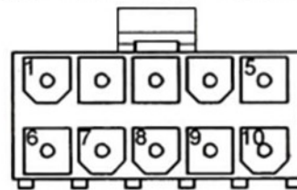
CONNECTOR VIEW FROM BACK SIDE
